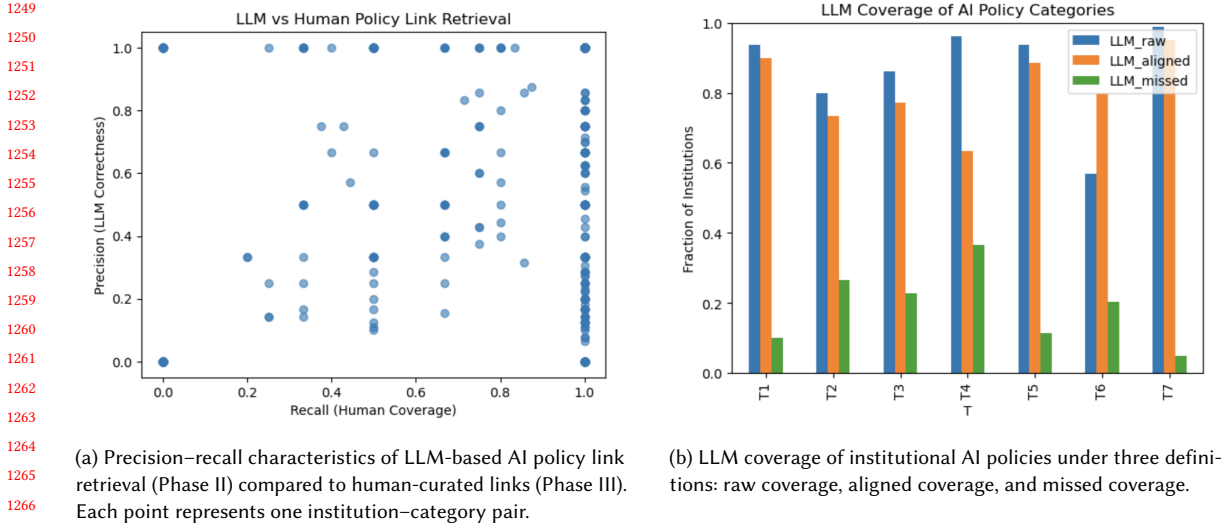
Fig. 7. Comparison of LLM-based and human-curated AI policy link retrieval.
