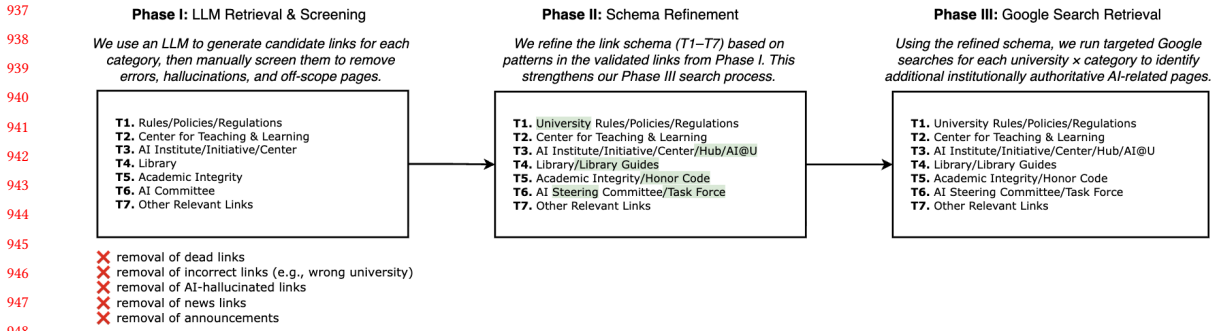
Fig. 5. Overview of Iterative Link Categorization Process: See Figure 6 for more details on Phases II and III.
